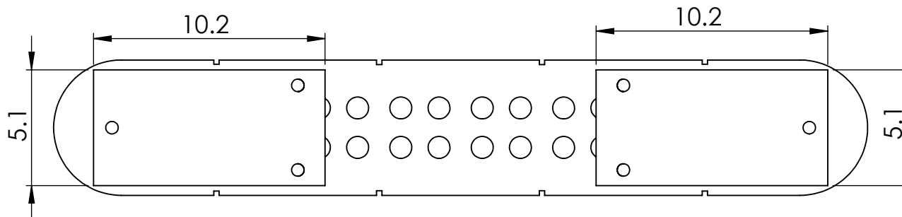
BOTTOM GLUE DOWN PLATE SIZE REQUIRES 1/12 QUART OF EPOXY
