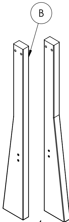
4 Table Legs
