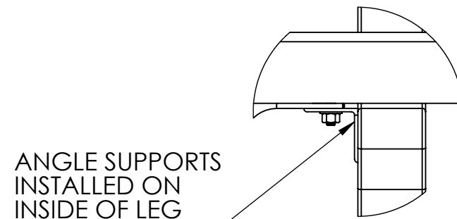
3 ASSEMBLY DETAIL
