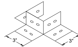
ANCHOR SHOE
