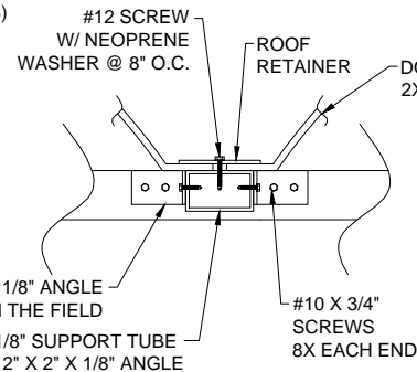
VIEW E-E
